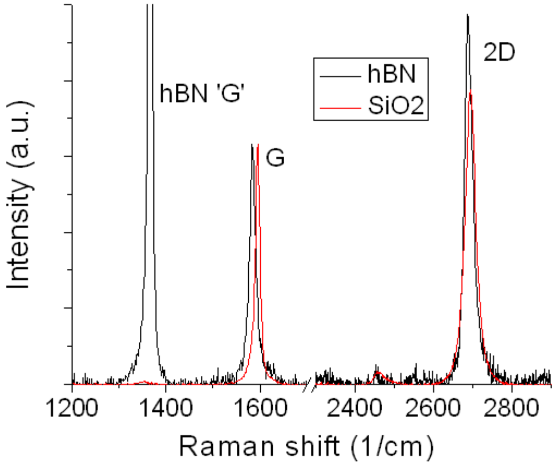
Figure 4.6: Raman spectra of hBN- and \text{SiO}_2 -supported graphene
