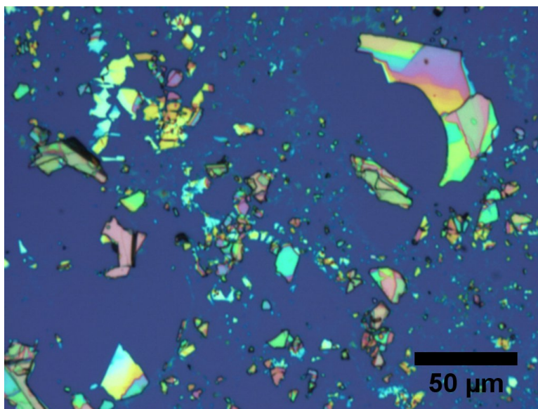
Figure 5.17: Tape exfoliated tin sulfide on 300nm SiO 2 on Si wafer
